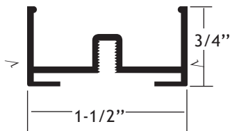
Part #170012 Jamb and Header Stock Length = 144"
