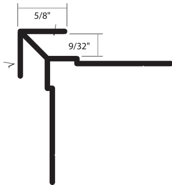
Part #120065 90° Column Trim
