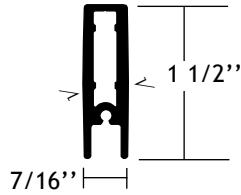
Part #110198 Face Frame
