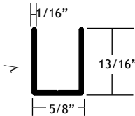
13/16" Single Channel
