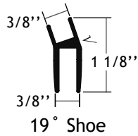
Part #110072
