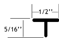
Part #110065
