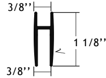
Part #110067
