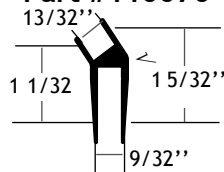
35° Deep Shoe
