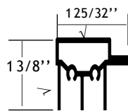
Part #110102
