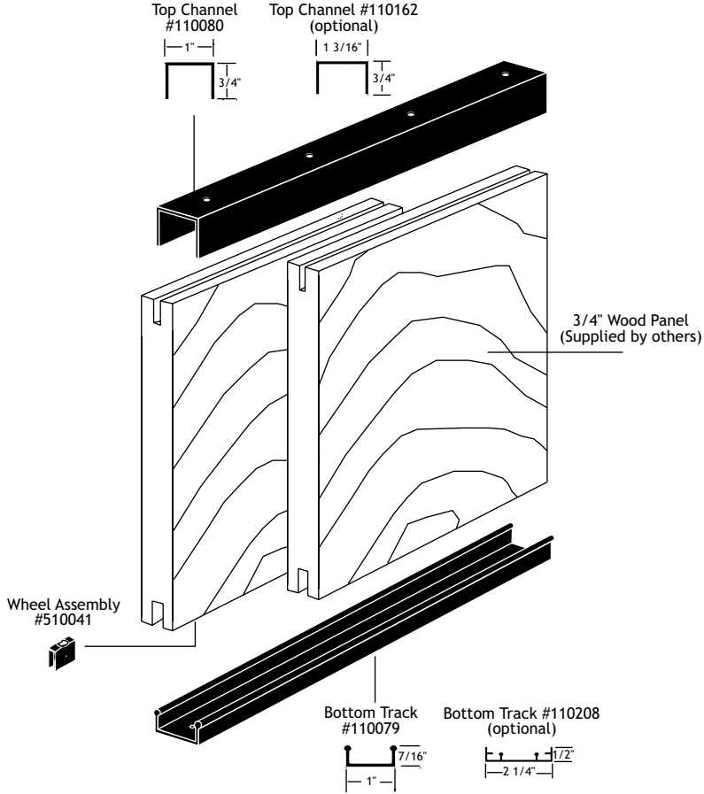
Model #610060 Double track for use when security is not required
