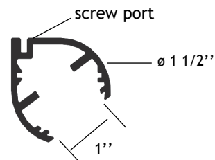
683900 series (screw port assembly)
