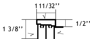
Part #110640 Backframe Header without Top Glass for 1/2" glass
