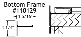
Standard profile bottom frame
