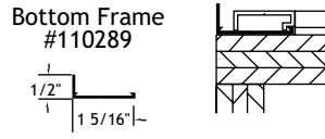
Low profile bottom frame
