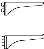
Part #550006 Aluminum Shelf Blade Bracket with and without Lip Available in 6, 8, 10, 12, 14, 16"
