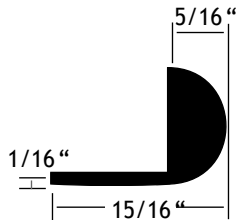
*Part # 110537 5/8" Half Round w/Leg
