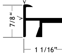
Part # 110192 Front Frame with Lip
