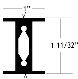
Part # 110106 Mullion
