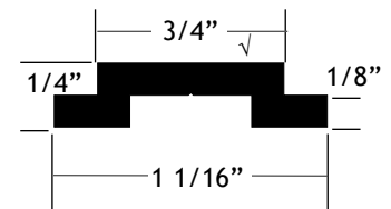
Part # 110391
