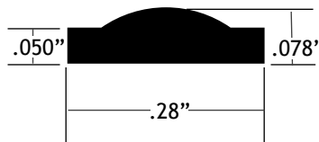
Part # 119006 Vinyl track insert works with #110035
