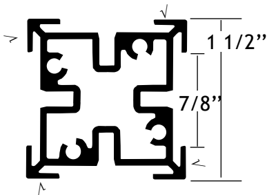
Part #170011 Corner Post Stock Length = 84"
