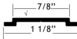
Part #170013 Corner Post Filler Strip Stock Length = 84"
