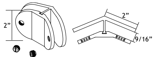
Part #510586 Round - 135° Clip
