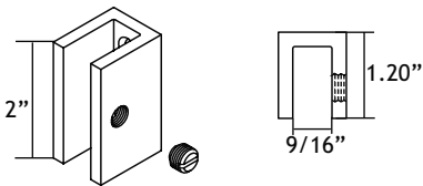
Part #510583 Square - 90° Wall Mount
