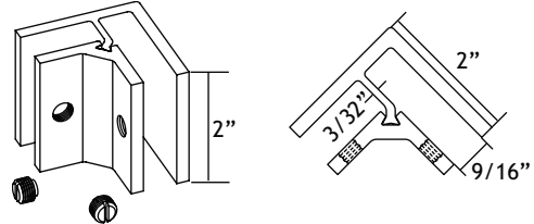
Part #510585 Square - 90° Clip
