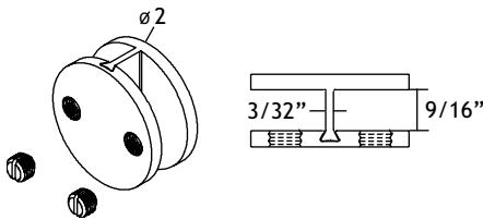
Part #510584 Round - 90° Clip
