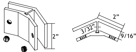
Part #510587 Square - 135° Clip
