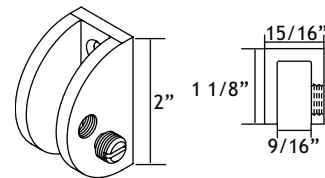
Part #510586 Round - 135° Clip
