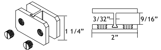
Part #510955 Rectangular - 180° Clip
