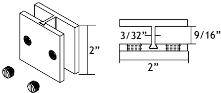
Part #510571 Square - 180° Clip
