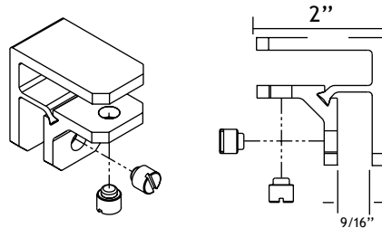
Part #511008 Rectangular - 90° Clip
