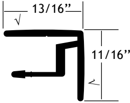
Part #120054 Mirror Frame
