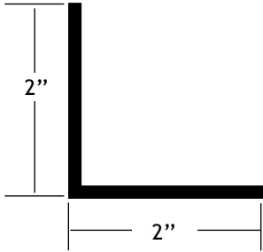
Part #110167 Angle Mount Bracket
