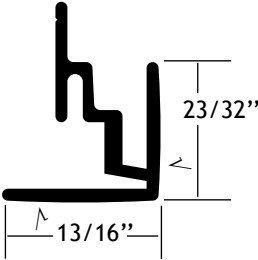
Part #120050 Mirror Frame - Bottom
