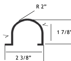
Part # 110741
