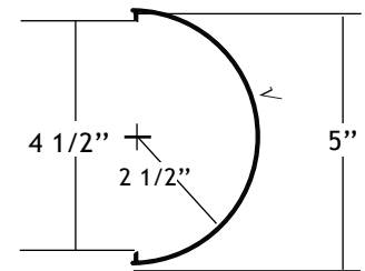
Part # 110211
