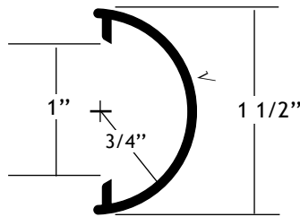
Part # 110200
